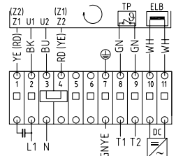
1-phase with brake
