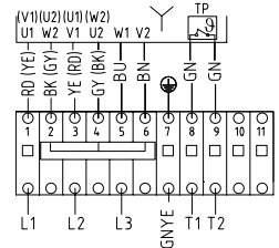
3-phase dual voltage star switch
