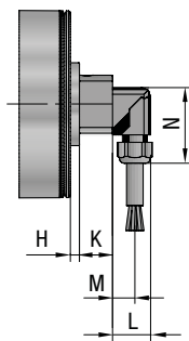
Elbow connector in polyamide
