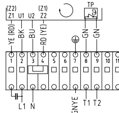
1-phase with brake
