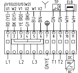
3-phase dual voltage star switch with brake
