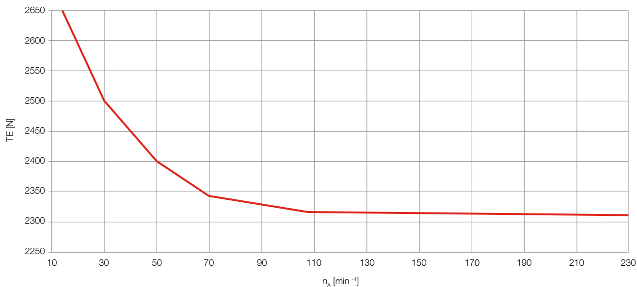
Belt tension depending on rated speed of shell
