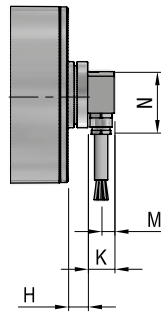
Cable connection 90°
