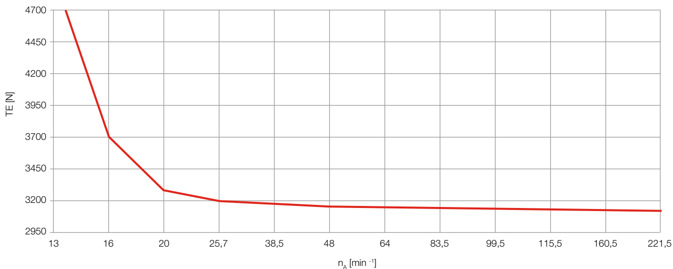
Belt tension depending on rated speed of shell
