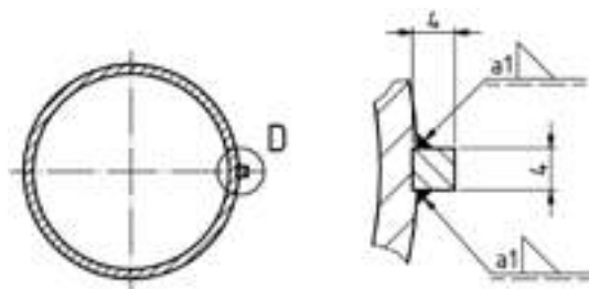
Drum motor with key 4x4
