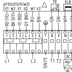
3-phase dual voltage delta switch with brake
