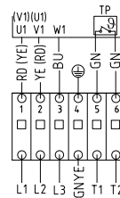
3-phase single voltage
