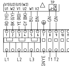
3-phase dual voltage delta switch
