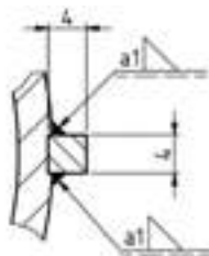
Drum motor with key 4x4
