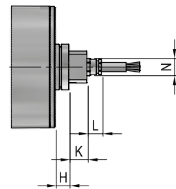
Straight connector
