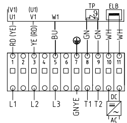
3-phase single voltage with brake
