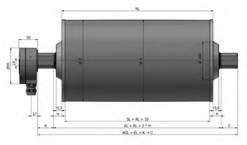
Drum motor standard version with terminal box in aluminium ≤ 4,0 kW
