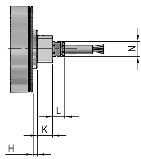
Straight connector
