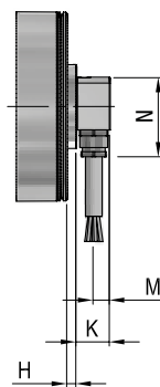
Cable connection 90°
