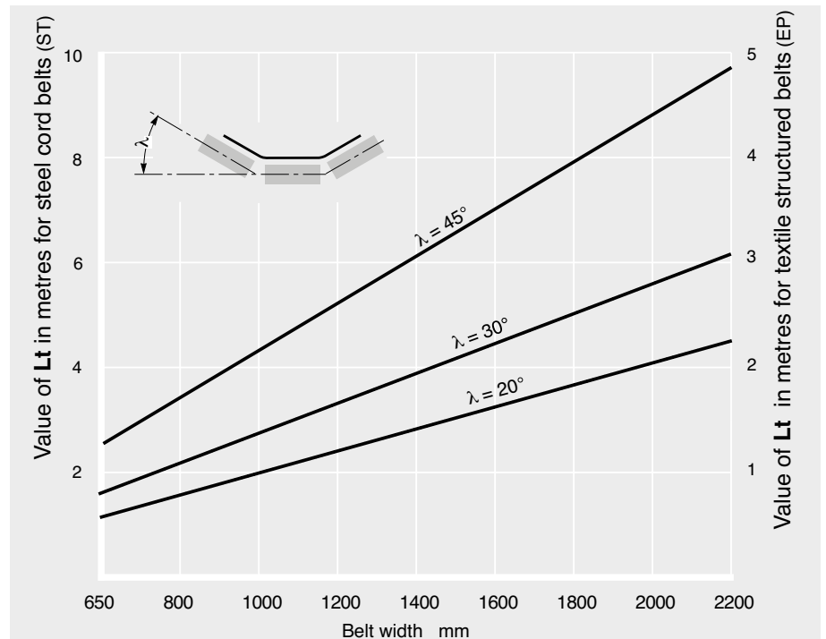
Fig.19 - Transition distance
