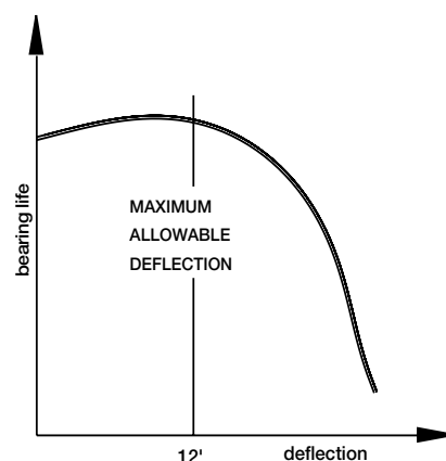
Fig. 3 - Deflection curve of bearings with C3 play.
