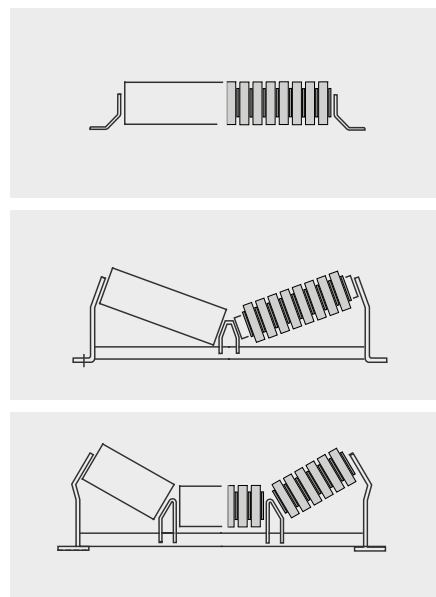
Fig. 1 - Fixed troughing sets
