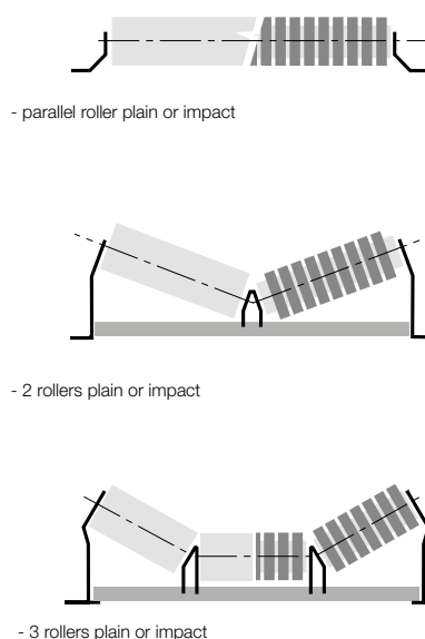
Fig. 9 - Troughing sets upper strand
