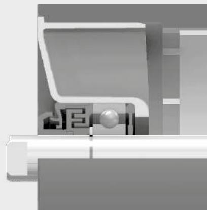
TOP C/1 Section through sealing
