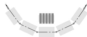
Fig. 8 - Suspended set for impact troughing set with three or five plain rollers or with shock absorbing rings
