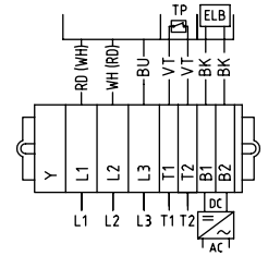
3-Ph motor single voltage with TP & ELB
