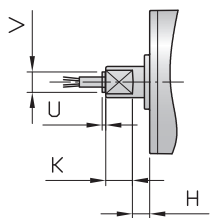
Straight connector
