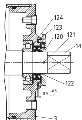
Labyrinth Option - Mild Steel
