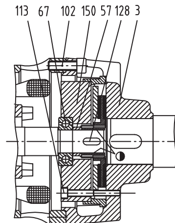
Electromagnetic brake
