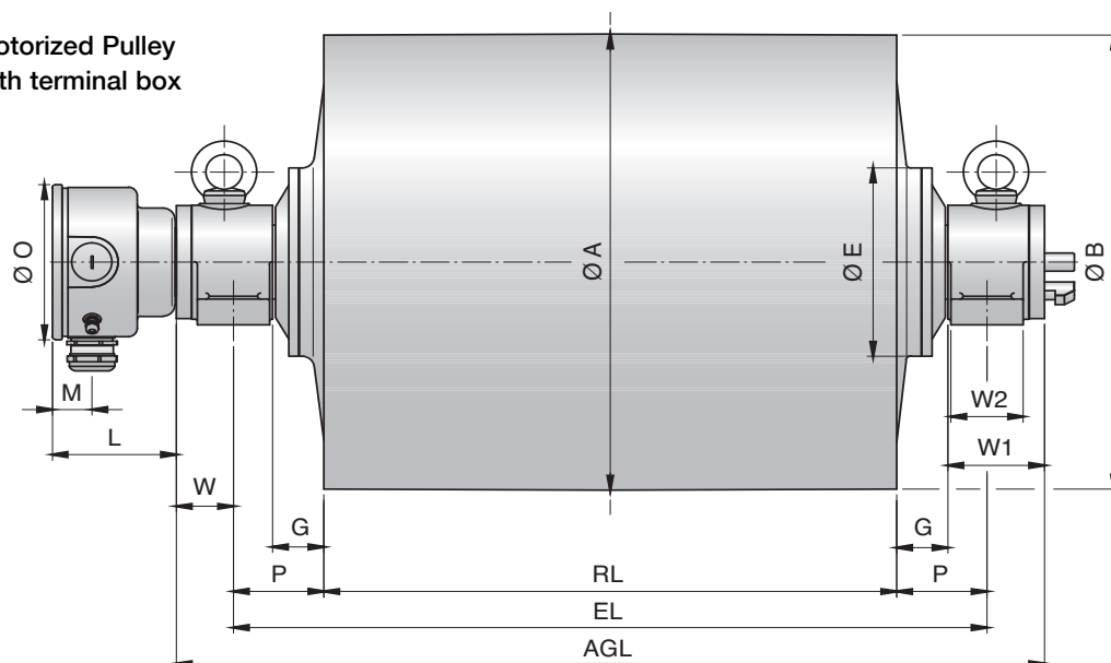
Idler Pulley UT630M / UT630H
