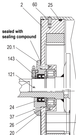
TS9N + TS11N Labyrinth Option valid for 320M
