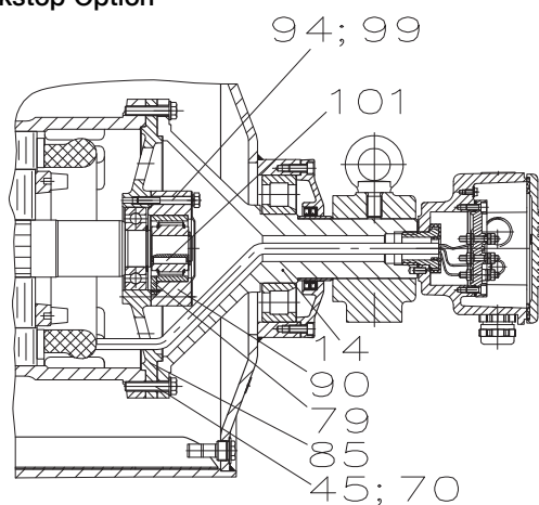
Backstop Option
