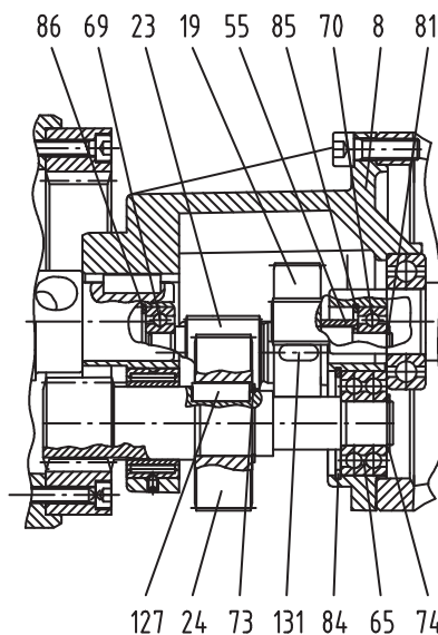
3-stage gearbox
