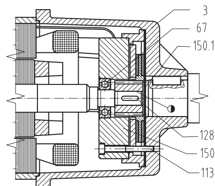
Electromagnetic brake
