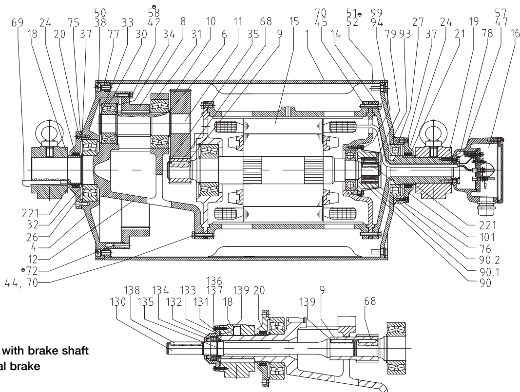
Backstop Execution
